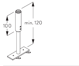
SG 6105 Hanger with plate
