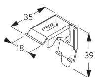
SG 2302 Bracket
