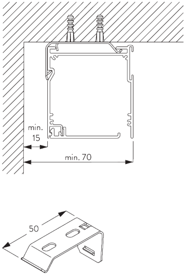
SG 2521 Bracket
