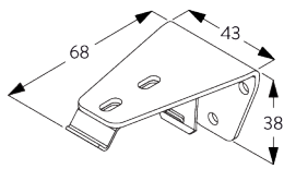
SG 2363 Bracket 68 mm
