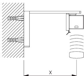
Smart Fix SG 11200 - SG 11203 and bracket SG 8201:
