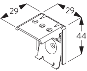
SG 8302 Bracket
